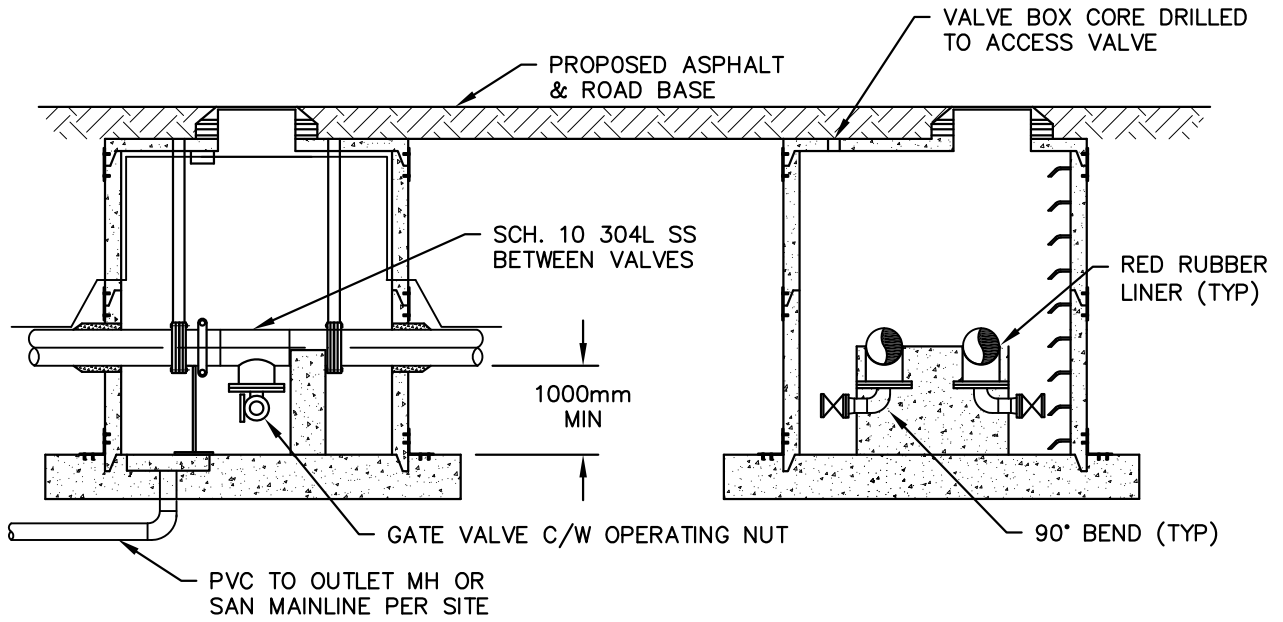
TERMINATION OF DRAIN AT SANITARY MANHOLE
