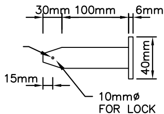
LOCKABLE PIN DETAIL
