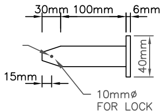
LOCKABLE PIN DETAIL
