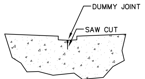
DETAIL OF C/L CONTROL JOINT
